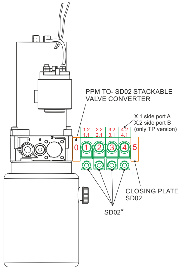
PPM + SD02 STACKABLE VALVES
