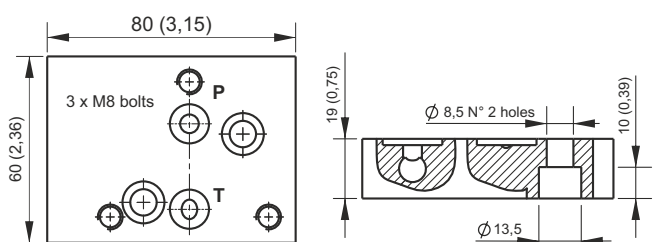
PPM TO SD02 STACKABLE VALVE CONVERTER (necessary to mount SD02 stackable valves)
