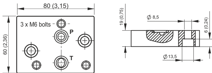
PPC TO SD02 STACKABLE VALVE CONVERTER (needed to mount SD02 stackable valves)
